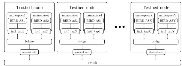
Fig. 3. BGP emulation toolchain architecture [3].
