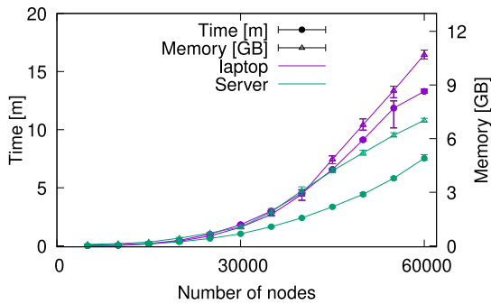
Fig. 8. Time (in minutes) and memory required to generate an Internet-like topology with our Python implementation versus the number of AS nodes. Results show the average (the dot), maximum and minimum (whisker) across 10 independent runs on an Intel i7 7500u (2.7–3.5 GHz) in purple, and across 50 independent runs on an Intel Xeon Silver (2.3 GHz) with 503 GB of memory in green.
