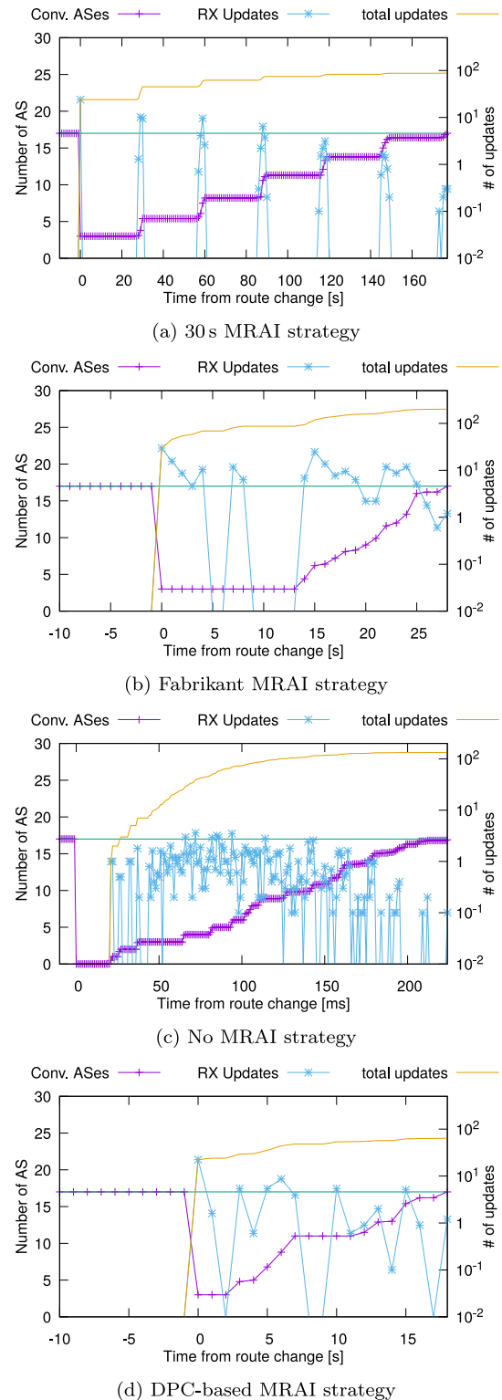
Fig. 4. Time evolution of MRAI strategies on a 17 nodes chain like the one in Fig. 1.
